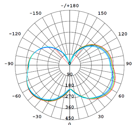
Distribution diagram (5000K)
