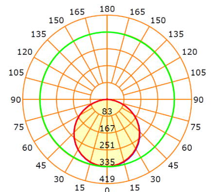
Distribution diagram (5000K)
